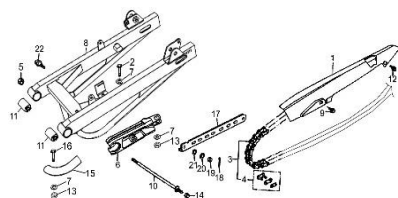
F21. REAR FORK / CHAIN CASE
