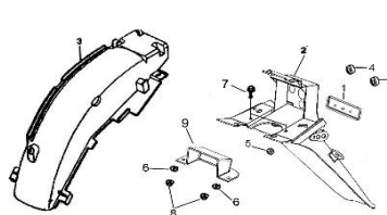
F23. REAR FENDER
