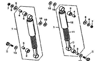
F22. REAR CUSHION
