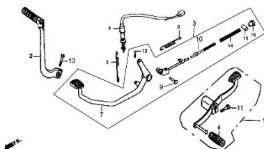
F18. PEDAL / KICK STARTER ARM
